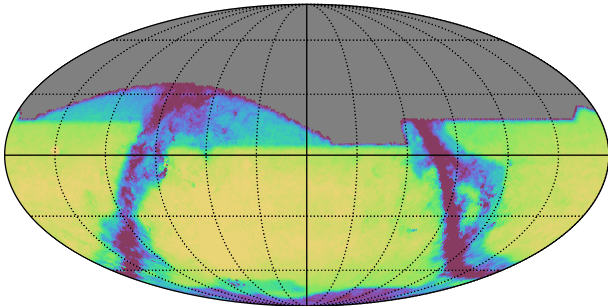
smc_lmc_v3.3_10yrs All sky z band: Exgal_CoaddM5
