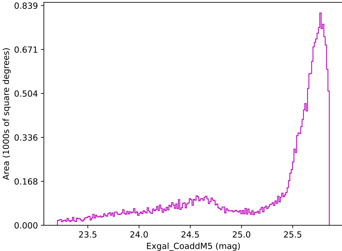
smc_lmc_v3.3_10yrs All sky z band: Exgal_CoaddM5
