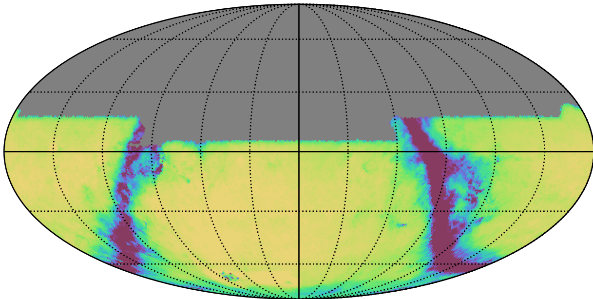
smc_lmc_v3.3_10yrs All sky u band: Exgal_CoaddM5
