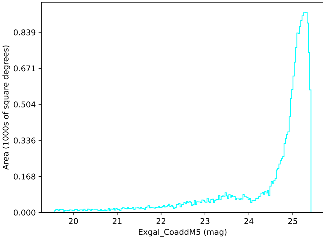
smc_lmc_v3.3_10yrs All sky u band: Exgal_CoaddM5
