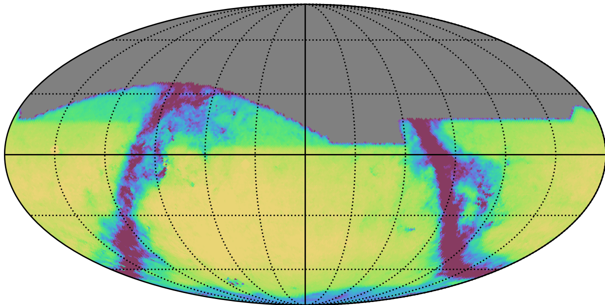
smc_lmc_v3.3_10yrs All sky r band: Exgal_CoaddM5
