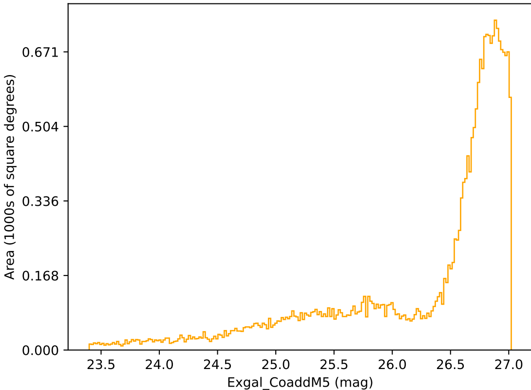
smc_lmc_v3.3_10yrs All sky r band: Exgal_CoaddM5
