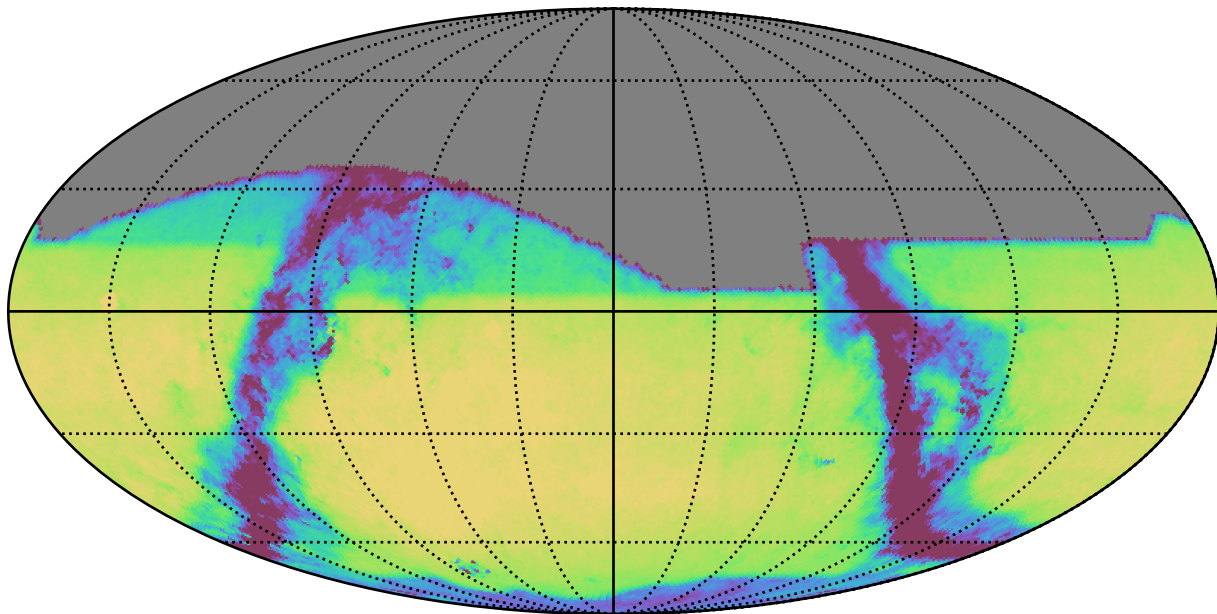
smc_lmc_v3.3_10yrs All sky i band: Exgal_CoaddM5
