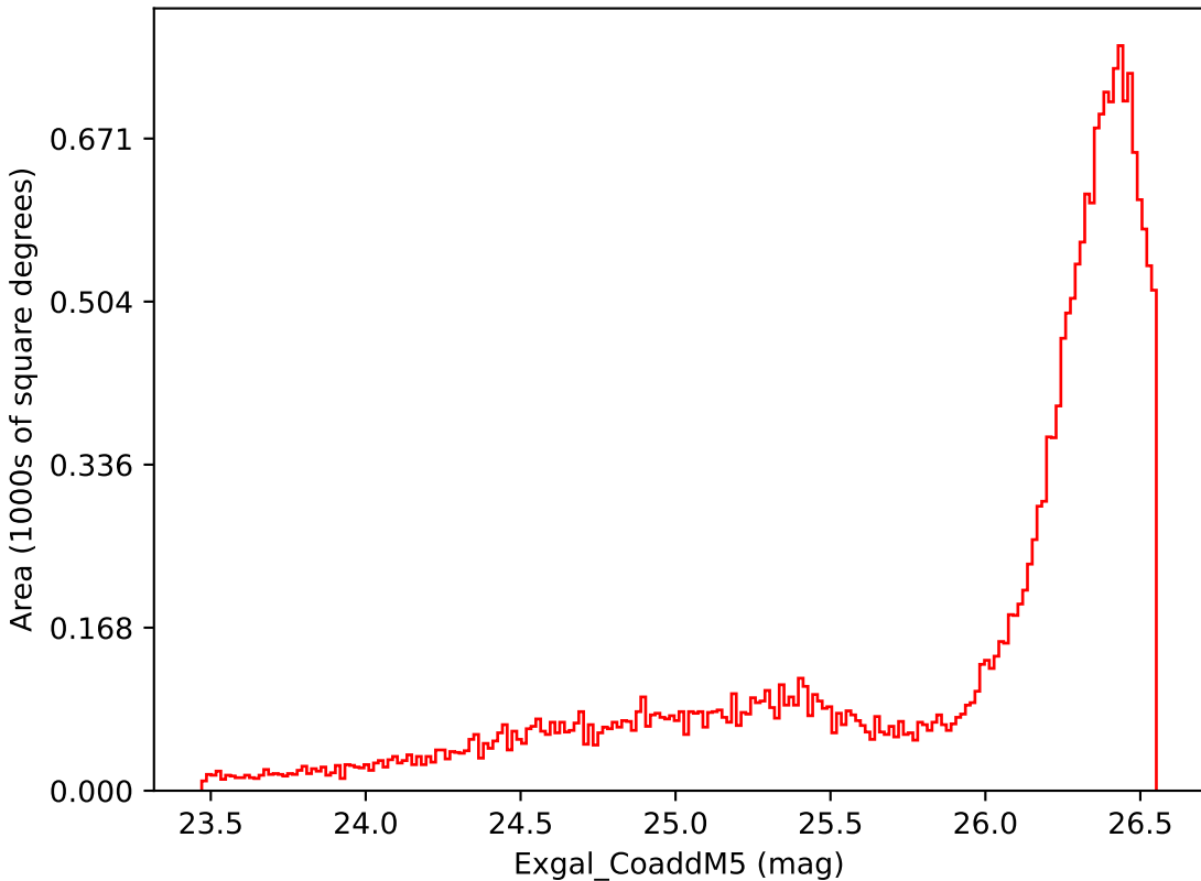
smc_lmc_v3.3_10yrs All sky i band: Exgal_CoaddM5
