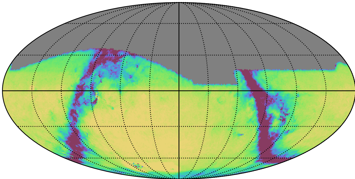
smc_lmc_v3.3_10yrs All sky g band: Exgal_CoaddM5
