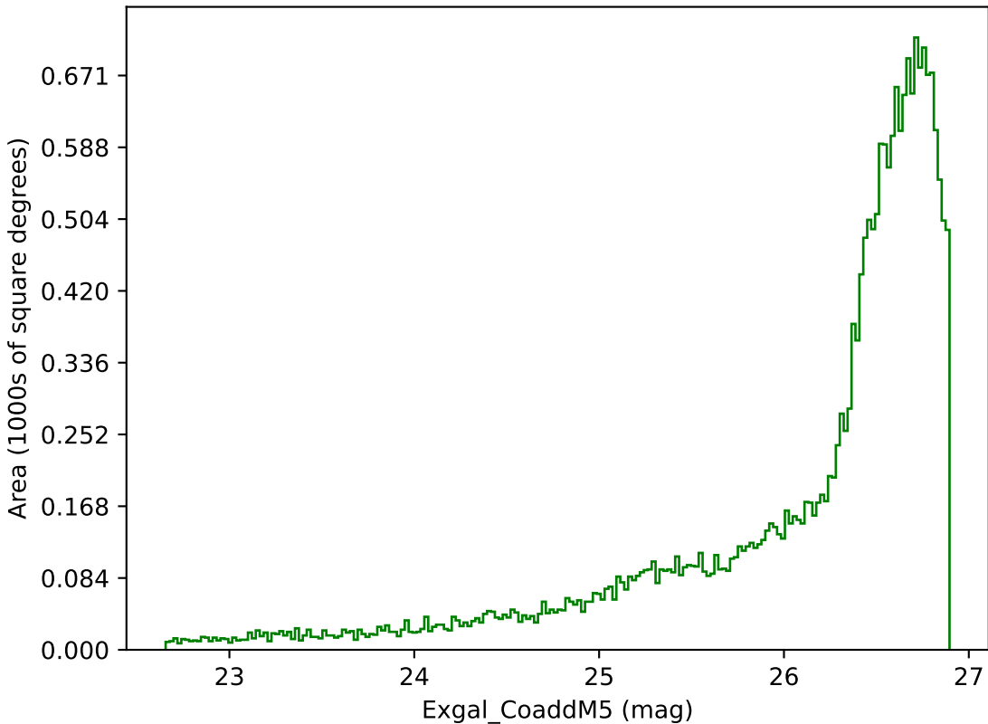
smc_lmc_v3.3_10yrs All sky g band: Exgal_CoaddM5
