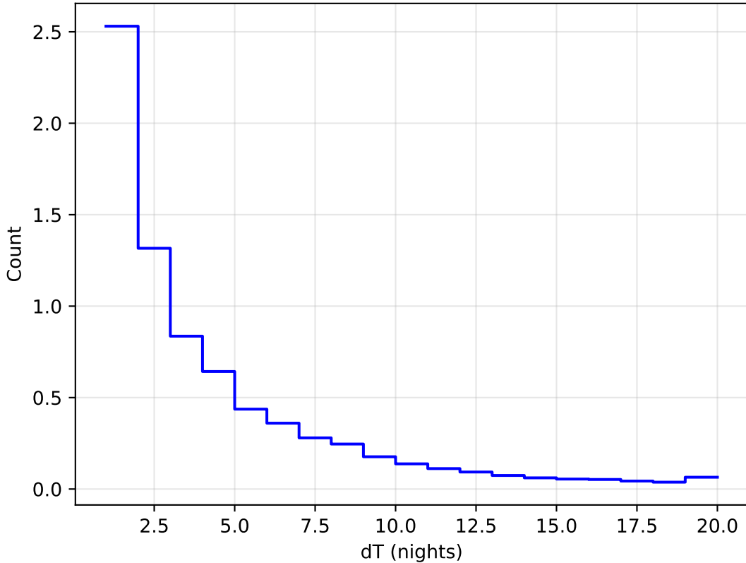
smc_lmc_v3.3_10yrs WFD all bands: DeltaNight Histogram 1e6
