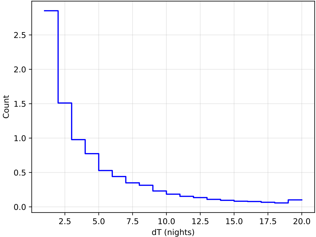
smc_lmc_v3.3_10yrs All sky all bands: DeltaNight Histogram 1e6
