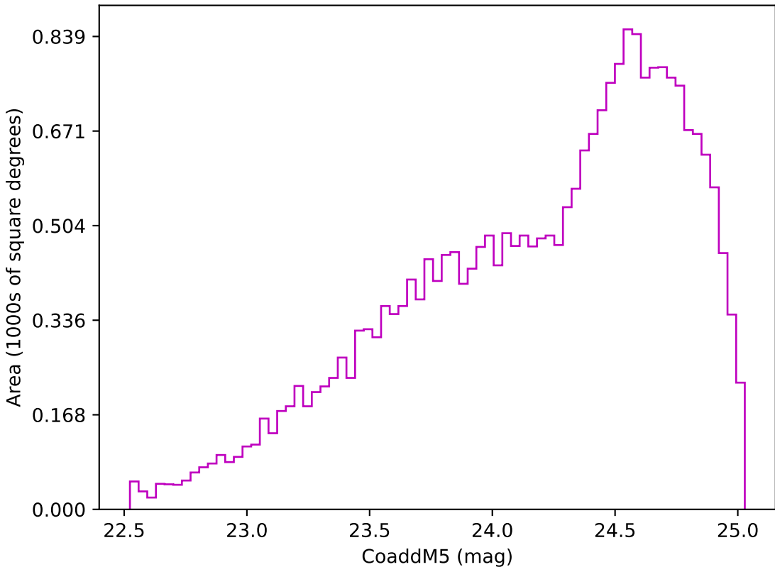
smc_lmc_v3.3_10yrs Yr 3-4 z band: CoaddM5
