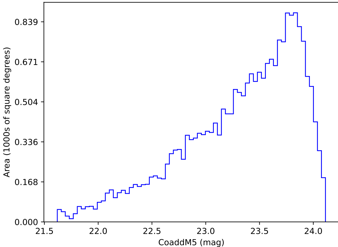
smc_lmc_v3.3_10yrs Yr 3-4 y band: CoaddM5
