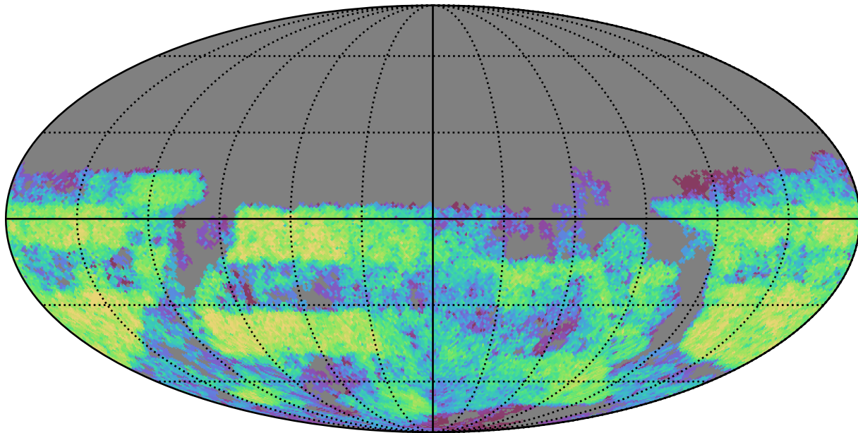
smc_lmc_v3.3_10yrs Yr 3-4 u band: CoaddM5
