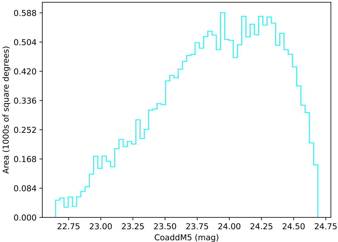
smc_lmc_v3.3_10yrs Yr 3-4 u band: CoaddM5
