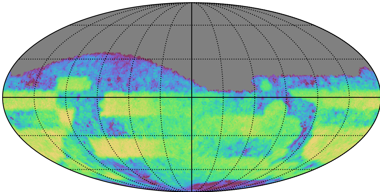
smc_lmc_v3.3_10yrs Yr 3-4 r band: CoaddM5
