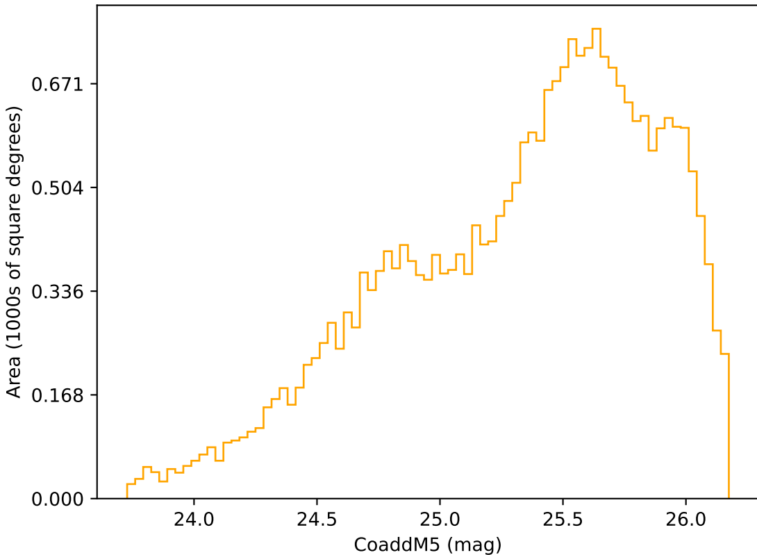
smc_lmc_v3.3_10yrs Yr 3-4 r band: CoaddM5
