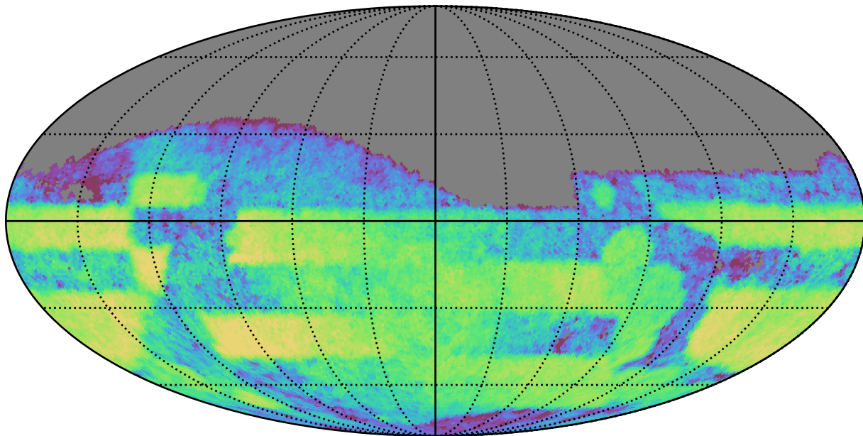
smc_lmc_v3.3_10yrs Yr 3-4 i band: CoaddM5
