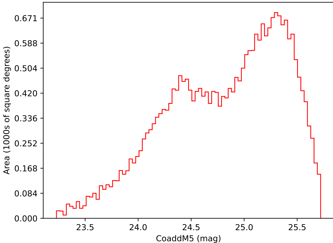
smc_lmc_v3.3_10yrs Yr 3-4 i band: CoaddM5
