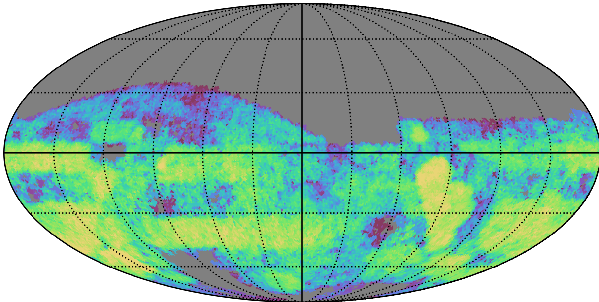
smc_lmc_v3.3_10yrs Yr 3-4 g band: CoaddM5
