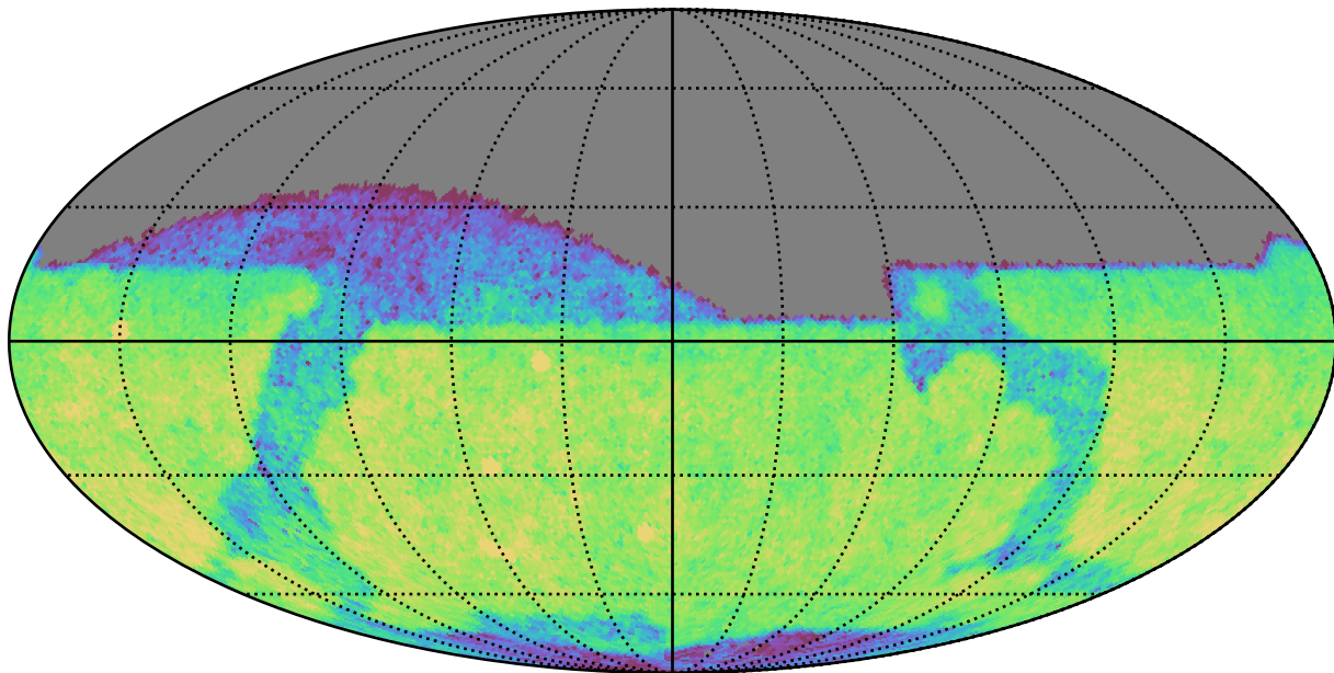
smc_lmc_v3.3_10yrs Yr 1 z band: CoaddM5
