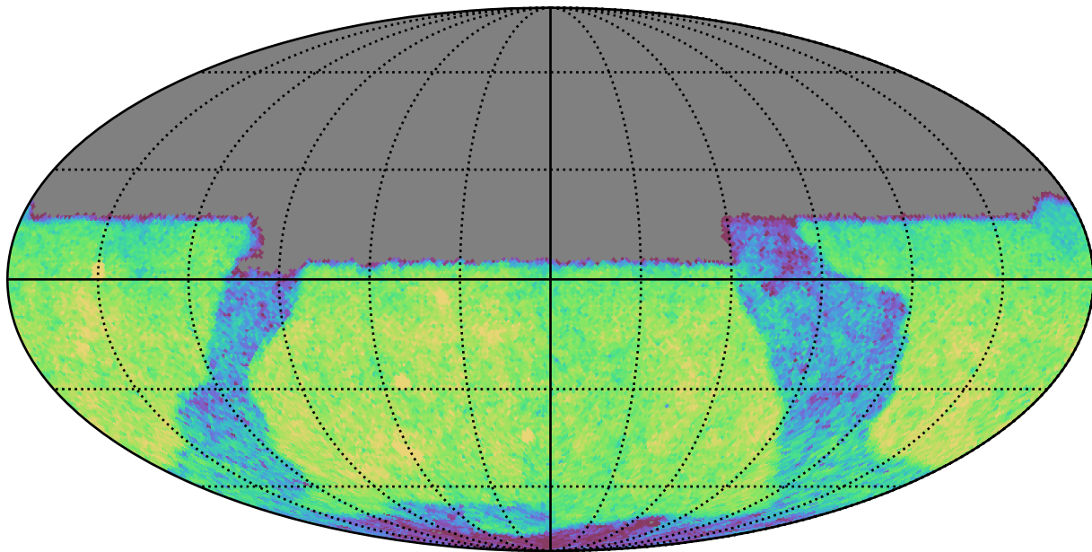
smc_lmc_v3.3_10yrs Yr 1 y band: CoaddM5
