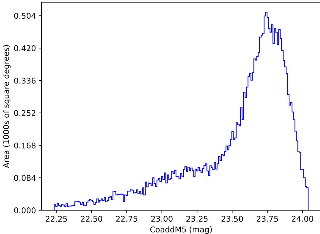
smc_lmc_v3.3_10yrs Yr 1 y band: CoaddM5
