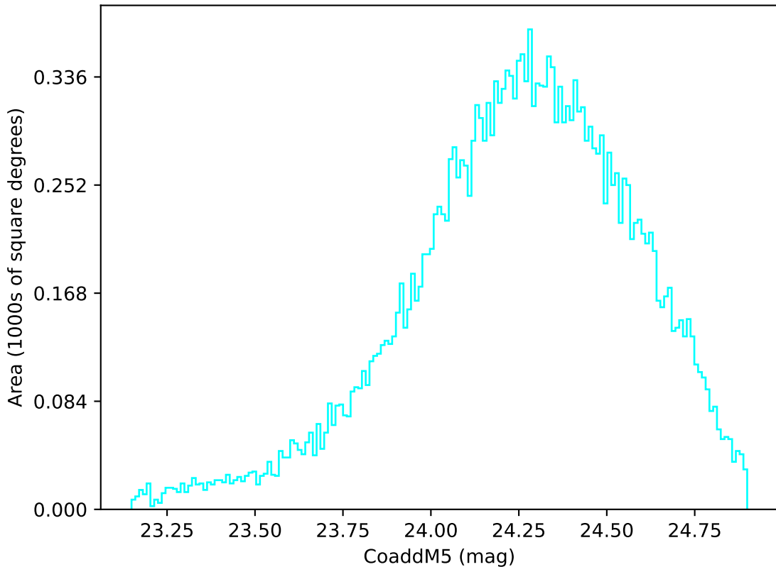
smc_lmc_v3.3_10yrs Yr 1 u band: CoaddM5
