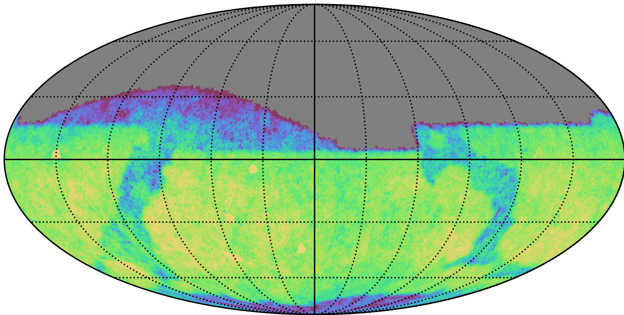
smc_lmc_v3.3_10yrs Yr 1 r band: CoaddM5
