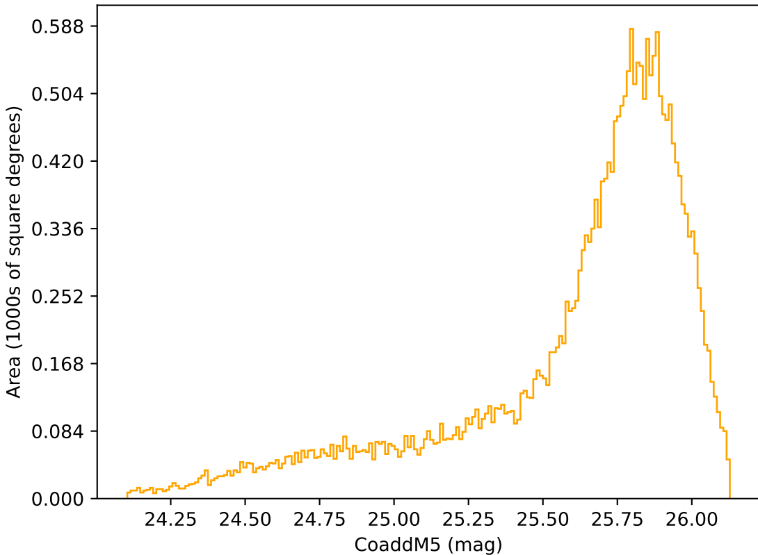
smc_lmc_v3.3_10yrs Yr 1 r band: CoaddM5
