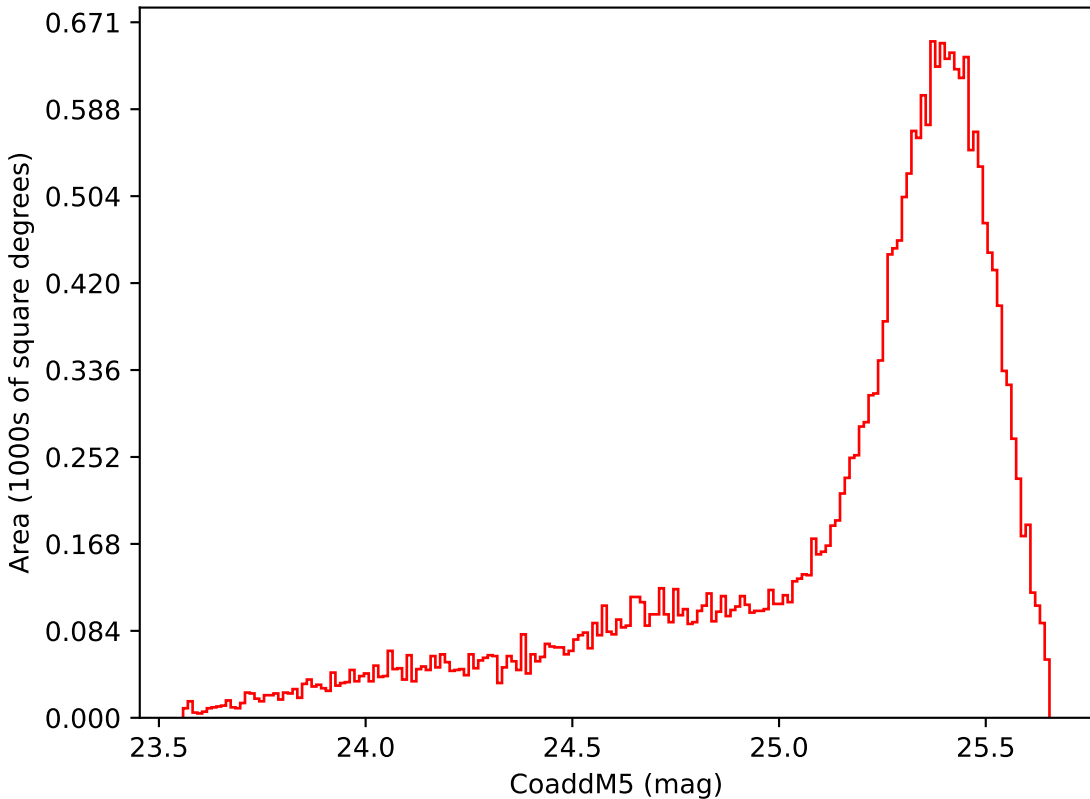
smc_lmc_v3.3_10yrs Yr 1 i band: CoaddM5
