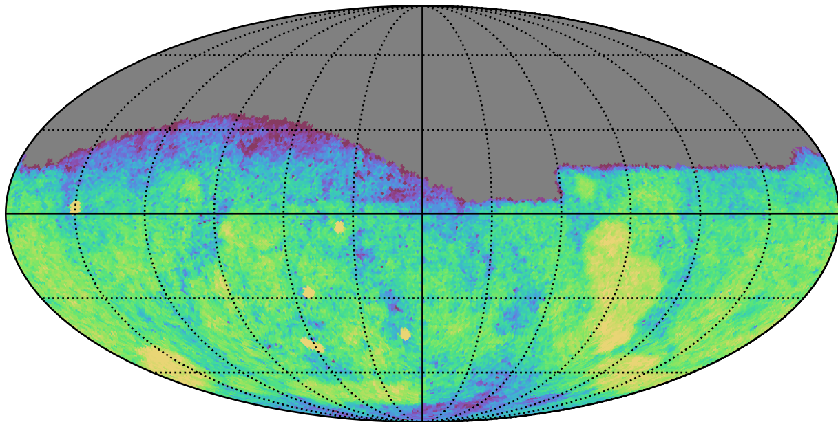
smc_lmc_v3.3_10yrs Yr 1 g band: CoaddM5
