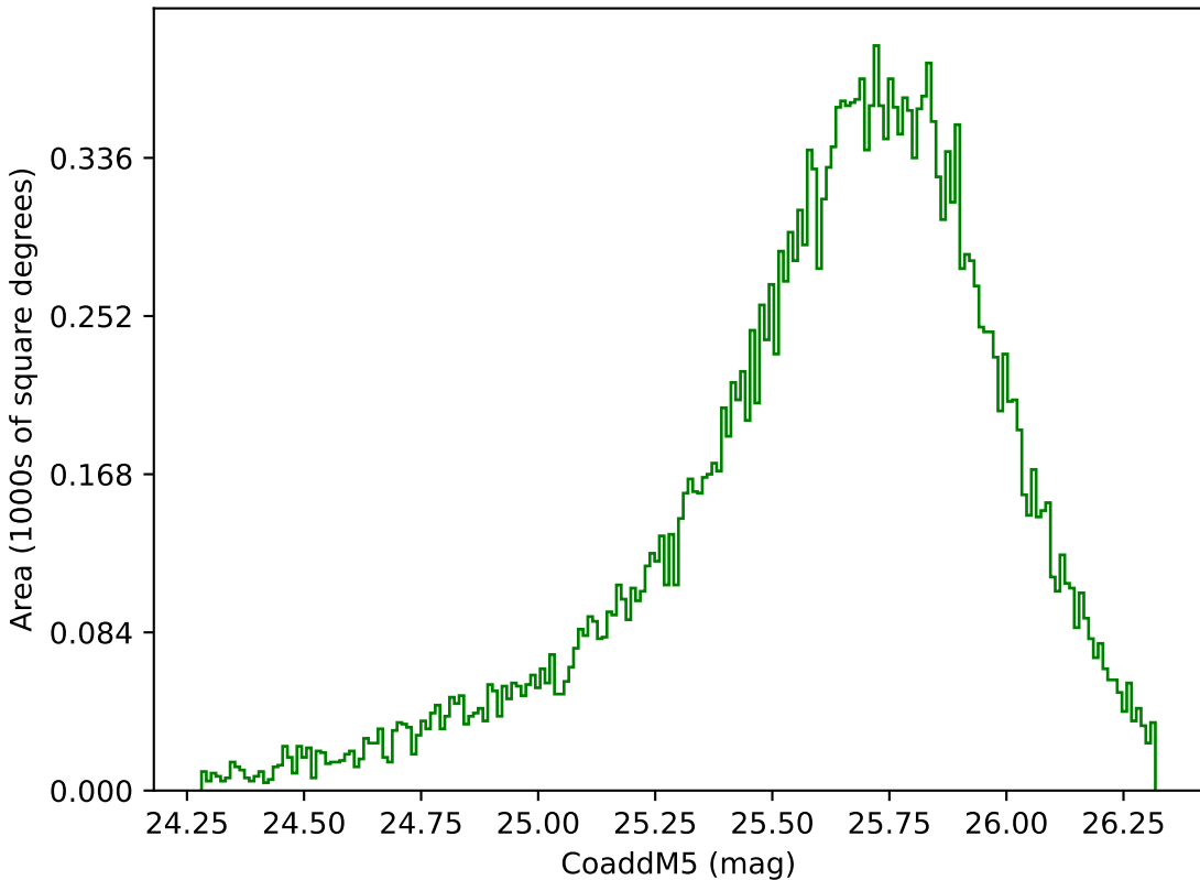
smc_lmc_v3.3_10yrs Yr 1 g band: CoaddM5
