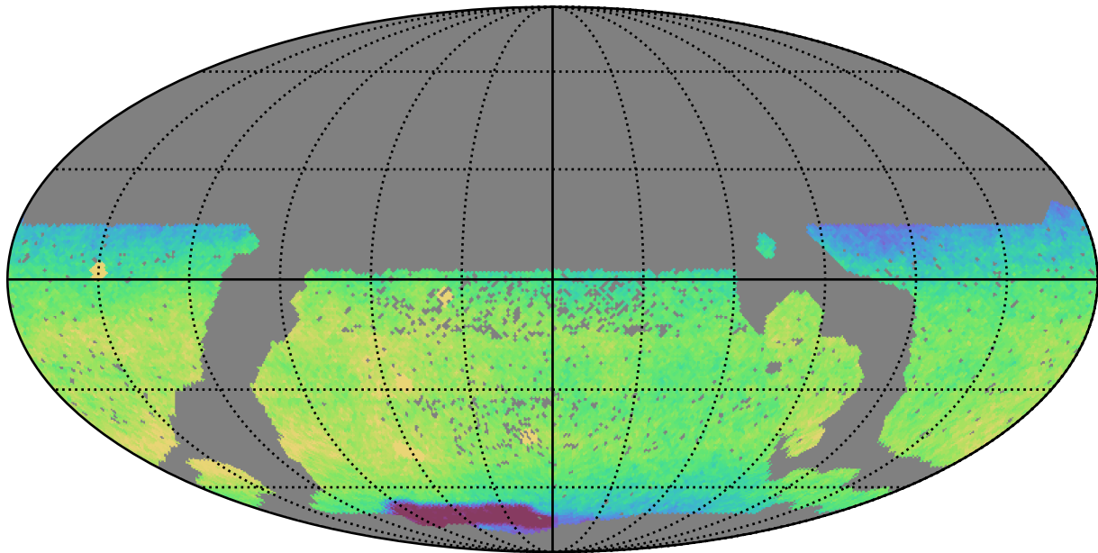
smc_lmc_v3.3_10yrs WFD z band: CoaddM5
