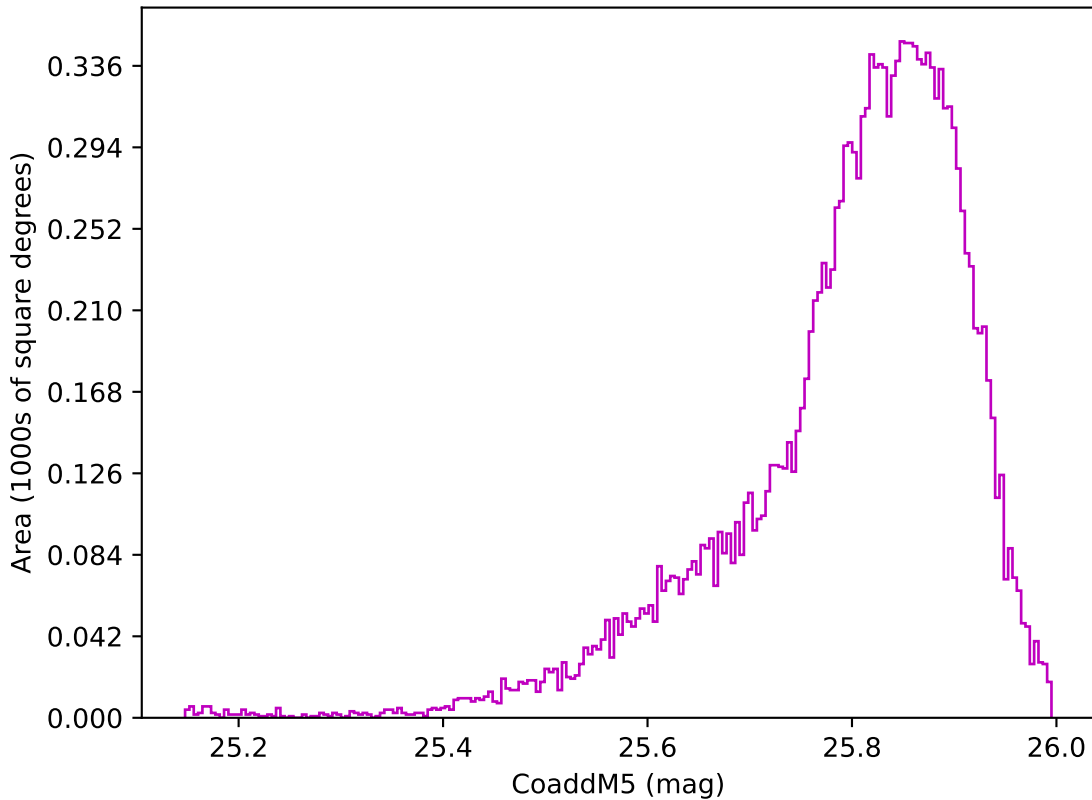
smc_lmc_v3.3_10yrs WFD z band: CoaddM5
