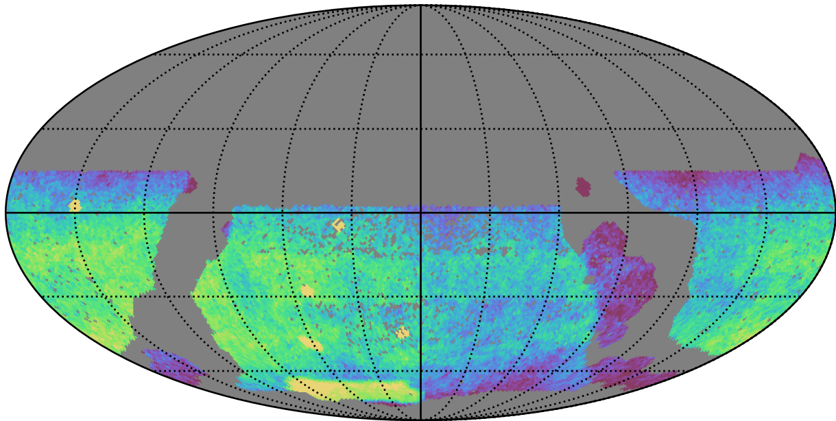
smc_lmc_v3.3_10yrs WFD u band: CoaddM5
