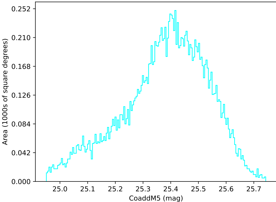
smc_lmc_v3.3_10yrs WFD u band: CoaddM5
