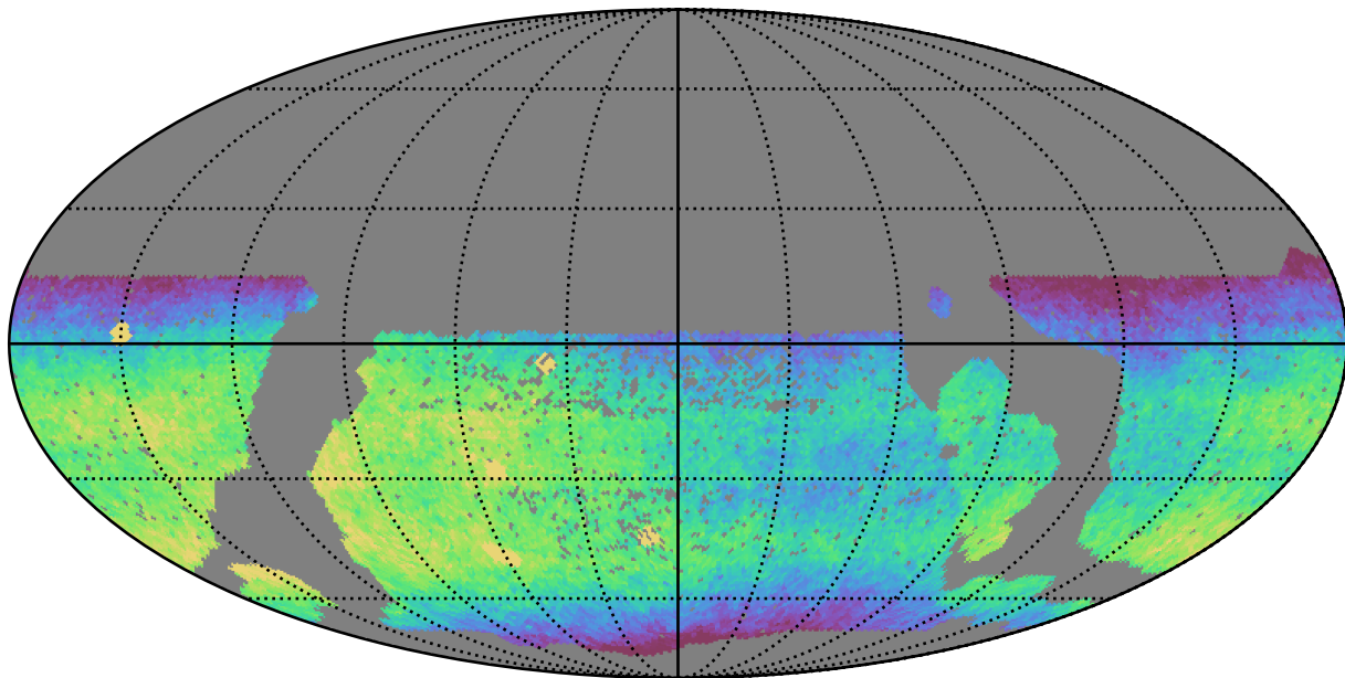
smc_lmc_v3.3_10yrs WFD r band: CoaddM5
