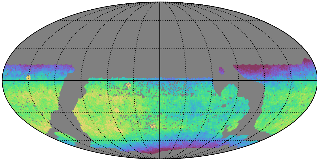
smc_lmc_v3.3_10yrs WFD i band: CoaddM5
