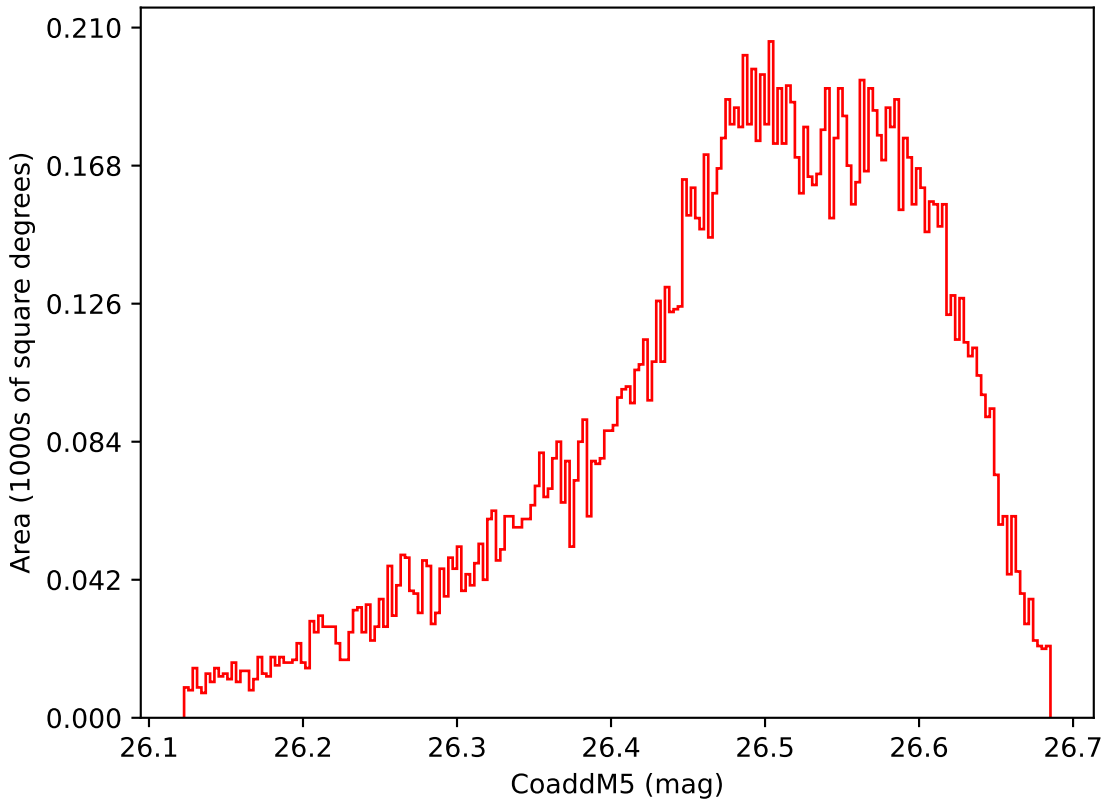
smc_lmc_v3.3_10yrs WFD i band: CoaddM5
