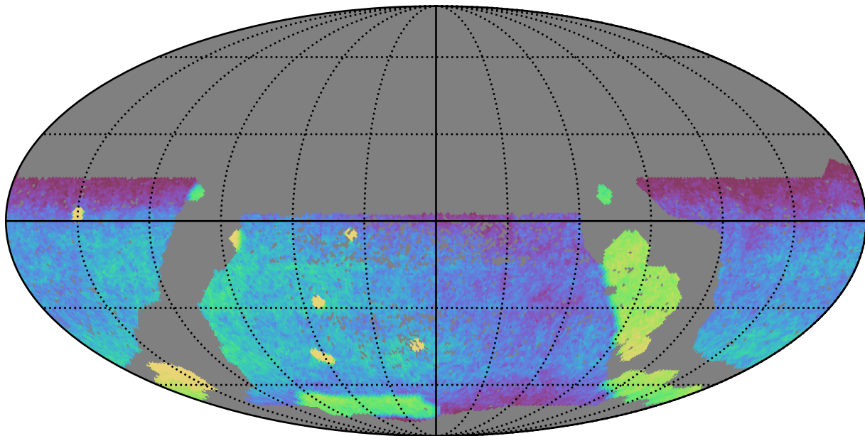
smc_lmc_v3.3_10yrs WFD g band: CoaddM5
