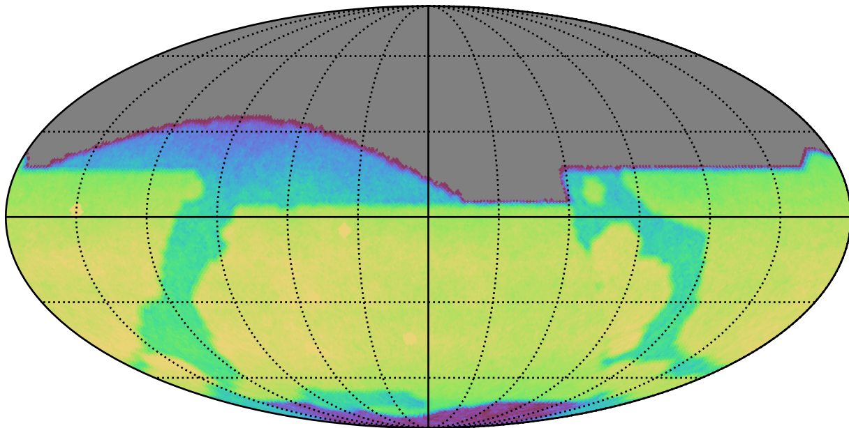
smc_lmc_v3.3_10yrs All sky z band: CoaddM5
