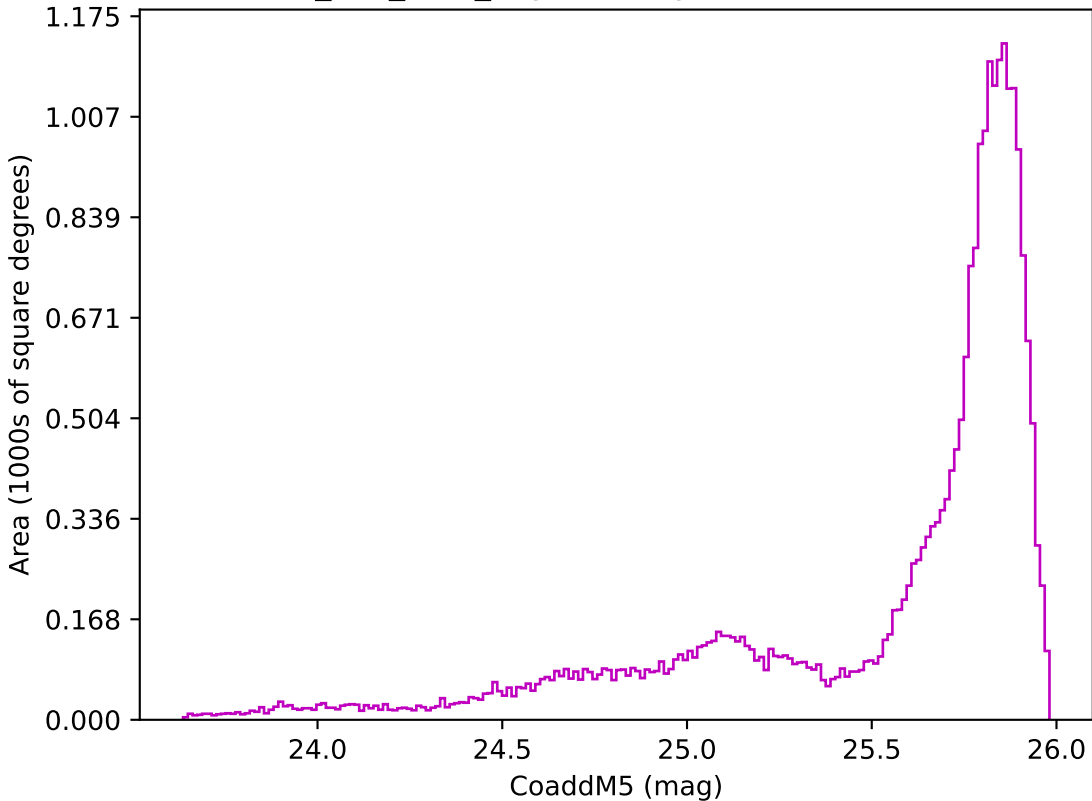
smc_lmc_v3.3_10yrs All sky z band: CoaddM5
