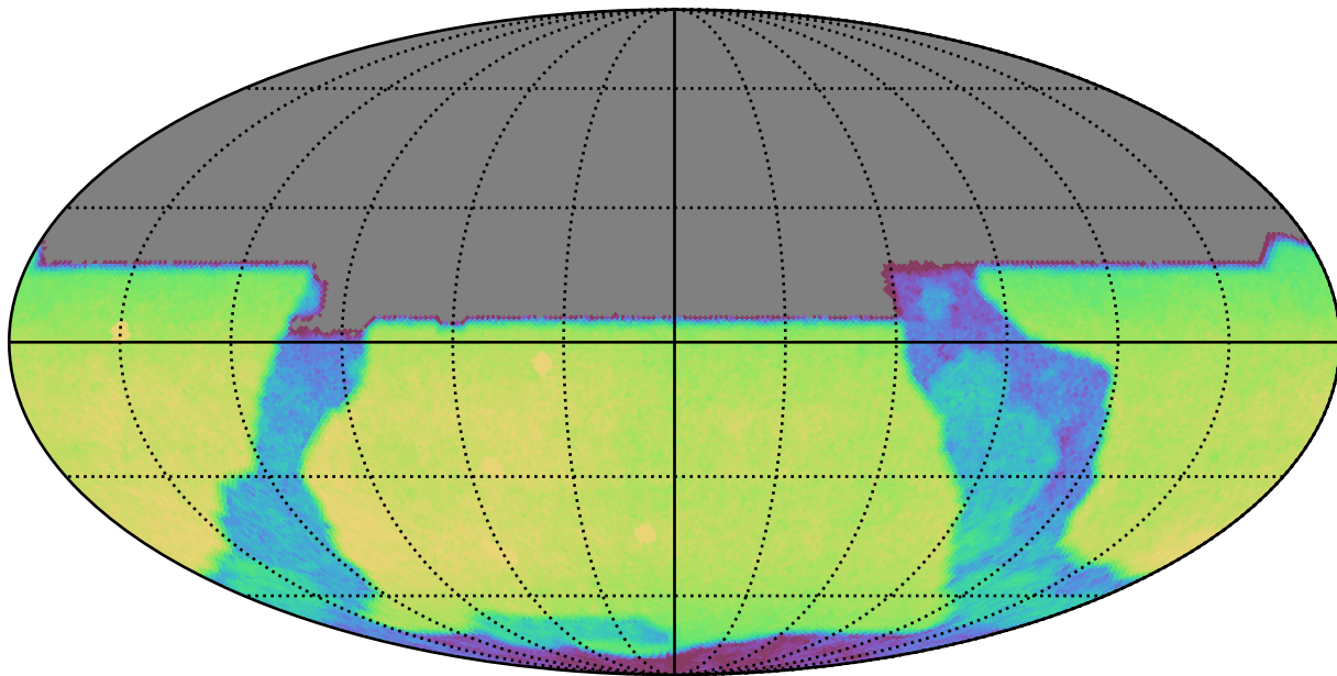
smc_lmc_v3.3_10yrs All sky y band: CoaddM5
