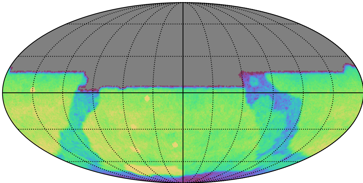
smc_lmc_v3.3_10yrs All sky u band: CoaddM5
