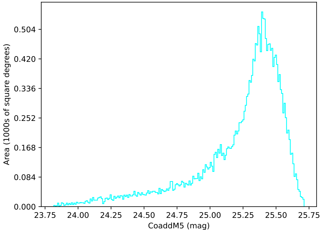
smc_lmc_v3.3_10yrs All sky u band: CoaddM5
