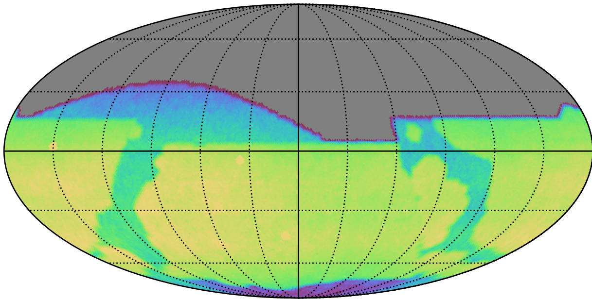
smc_lmc_v3.3_10yrs All sky r band: CoaddM5
