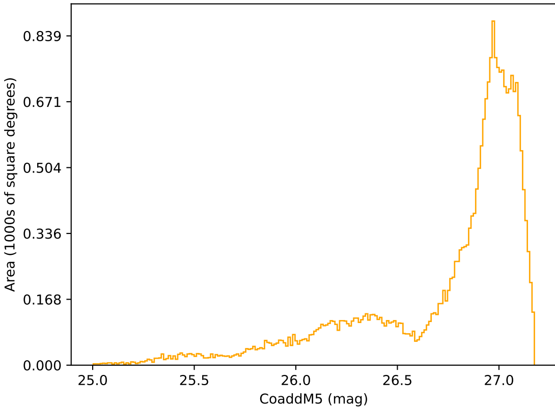
smc_lmc_v3.3_10yrs All sky r band: CoaddM5
