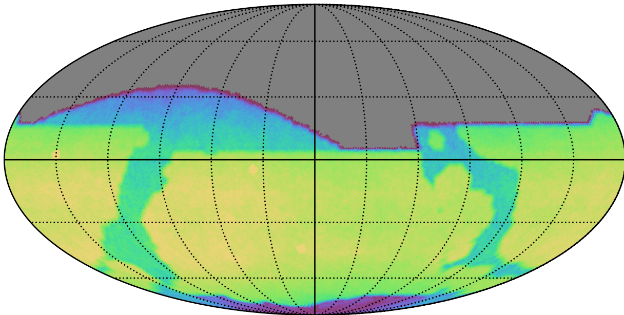
smc_lmc_v3.3_10yrs All sky i band: CoaddM5
