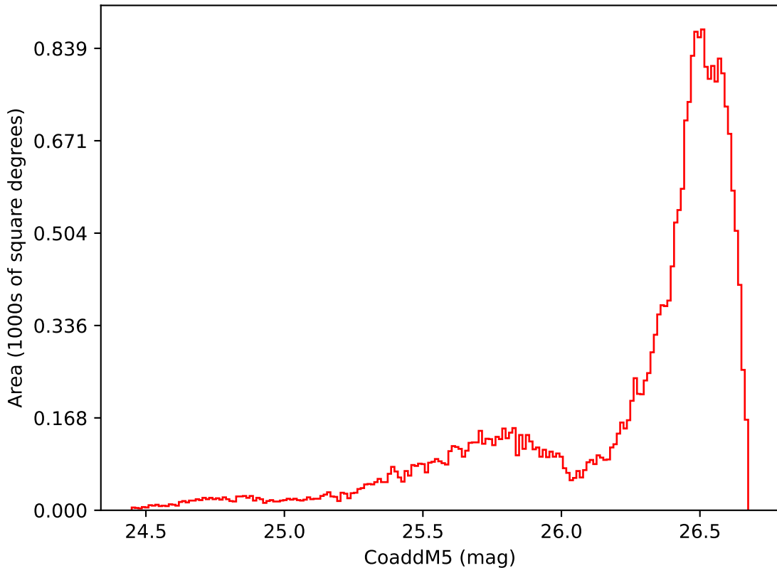
smc_lmc_v3.3_10yrs All sky i band: CoaddM5
