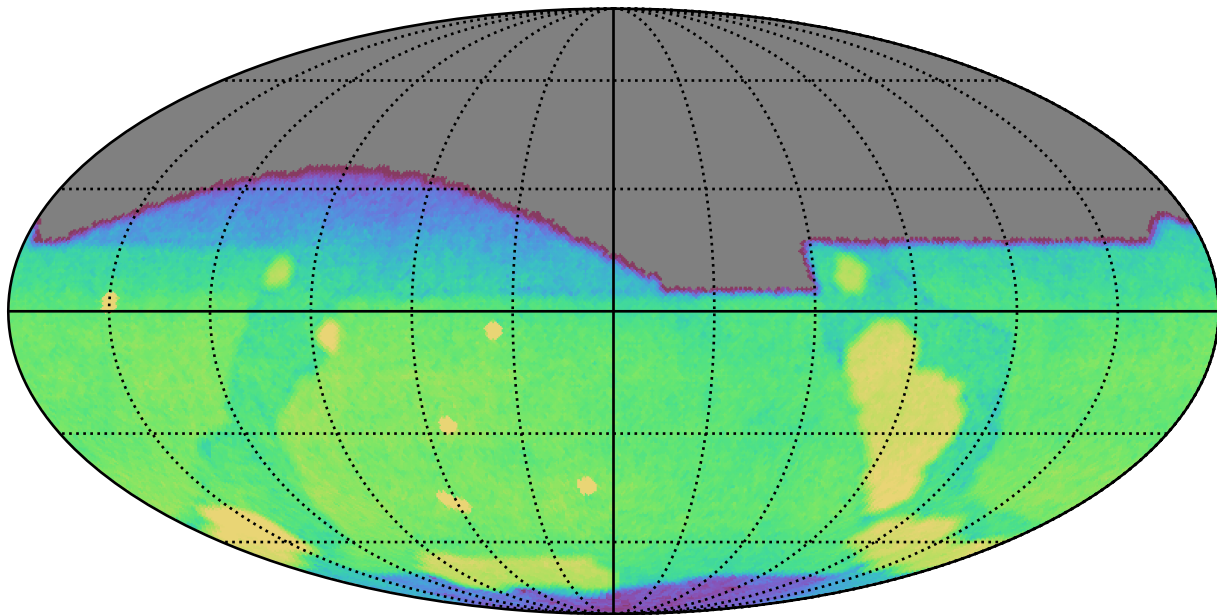
smc_lmc_v3.3_10yrs All sky g band: CoaddM5
