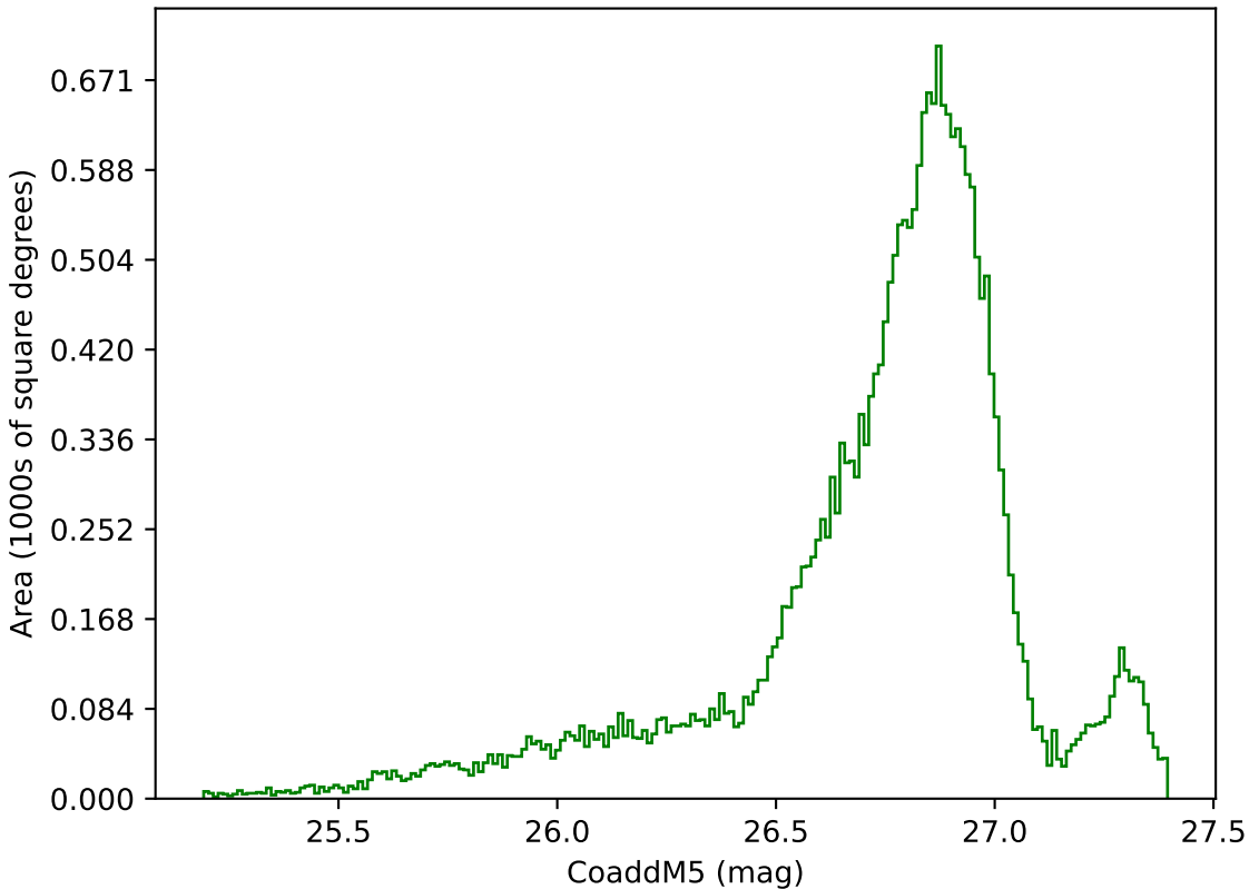
smc_lmc_v3.3_10yrs All sky g band: CoaddM5
