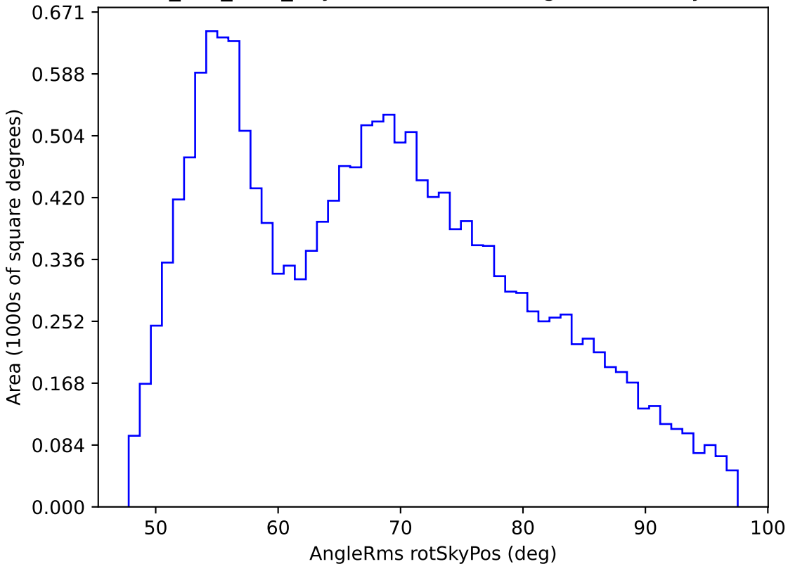
smc_lmc_v3.3_10yrs WFD z band: AngleRms rotSkyPos
